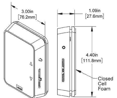
Standard Mounting Base
