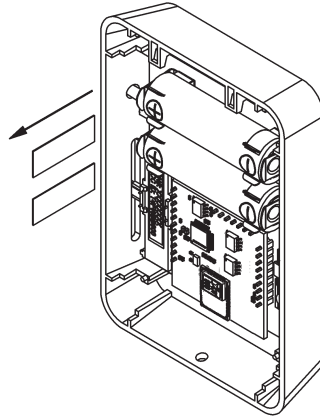
Fig. 2: Battery insulator tab removal
