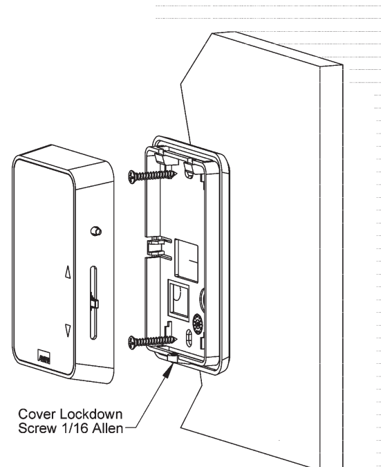
Fig. 4: BAPI-Stat “Quantum” Mounting
