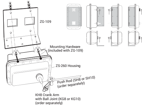
Typical ZG-109 Mounting
