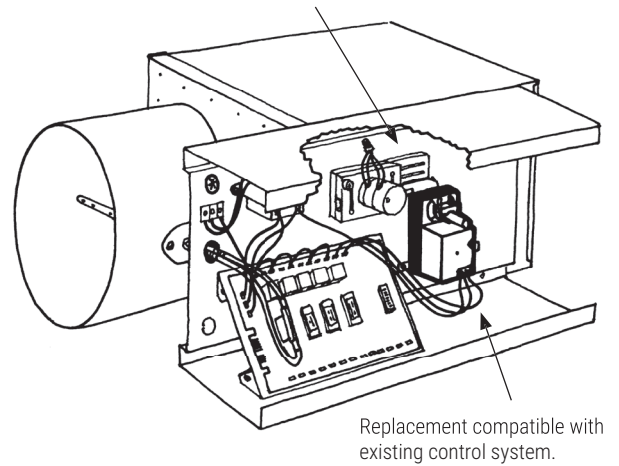
Figure 2.20: Actuator mounted in VAV box replacing rack and pinion type actuator
