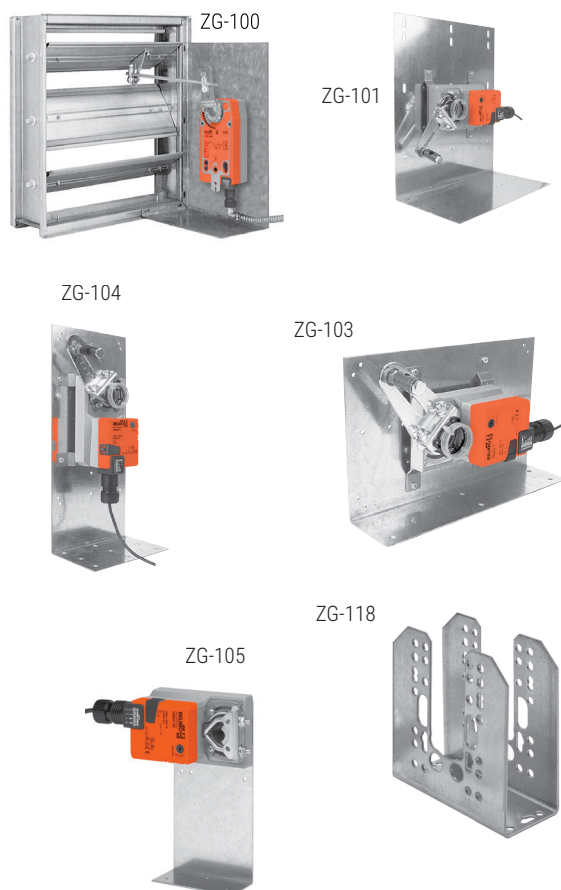
Figure 1.6: mounting brackets; for use when direct coupling is impossible
