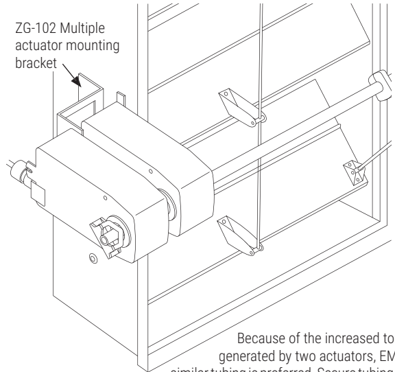
Figure 2.12: Multiple actuators mounted to a jackshaft
