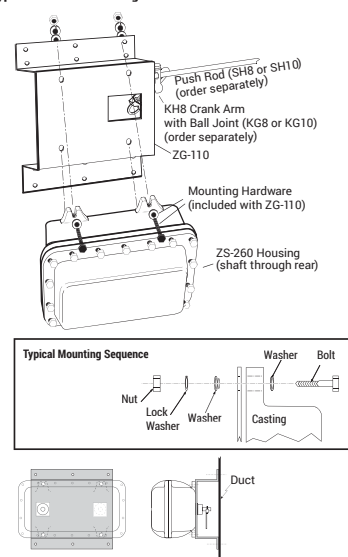
Typical ZG-110 Mounting
