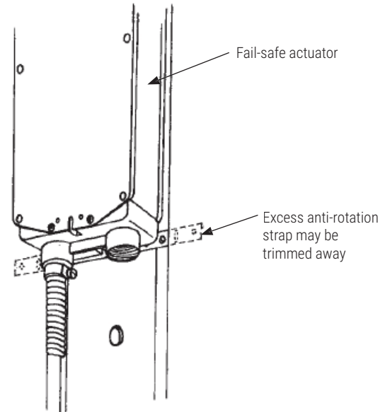
Figure 1.4: Modification of the anti-rotation strap
