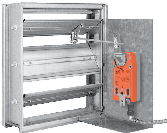
Figure 3.2: Universal mounting bracket is attached to the damper assembly
