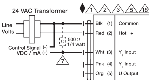
VDC/mA Control
