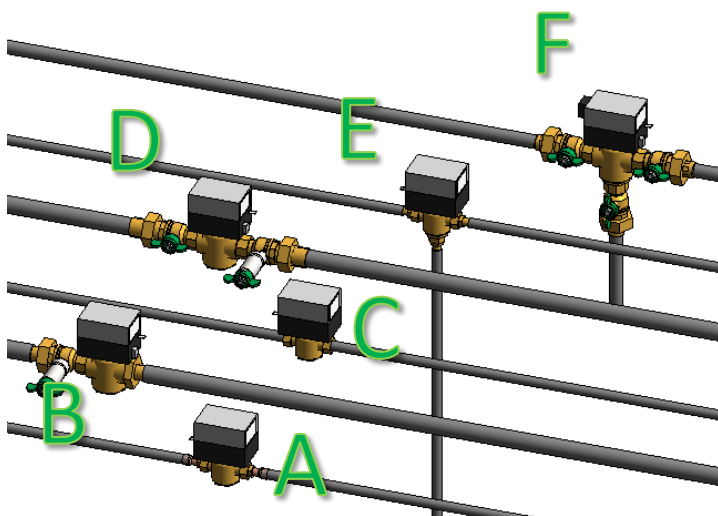
Figure 3 - OBCaleffi Z-One Zone Valves
