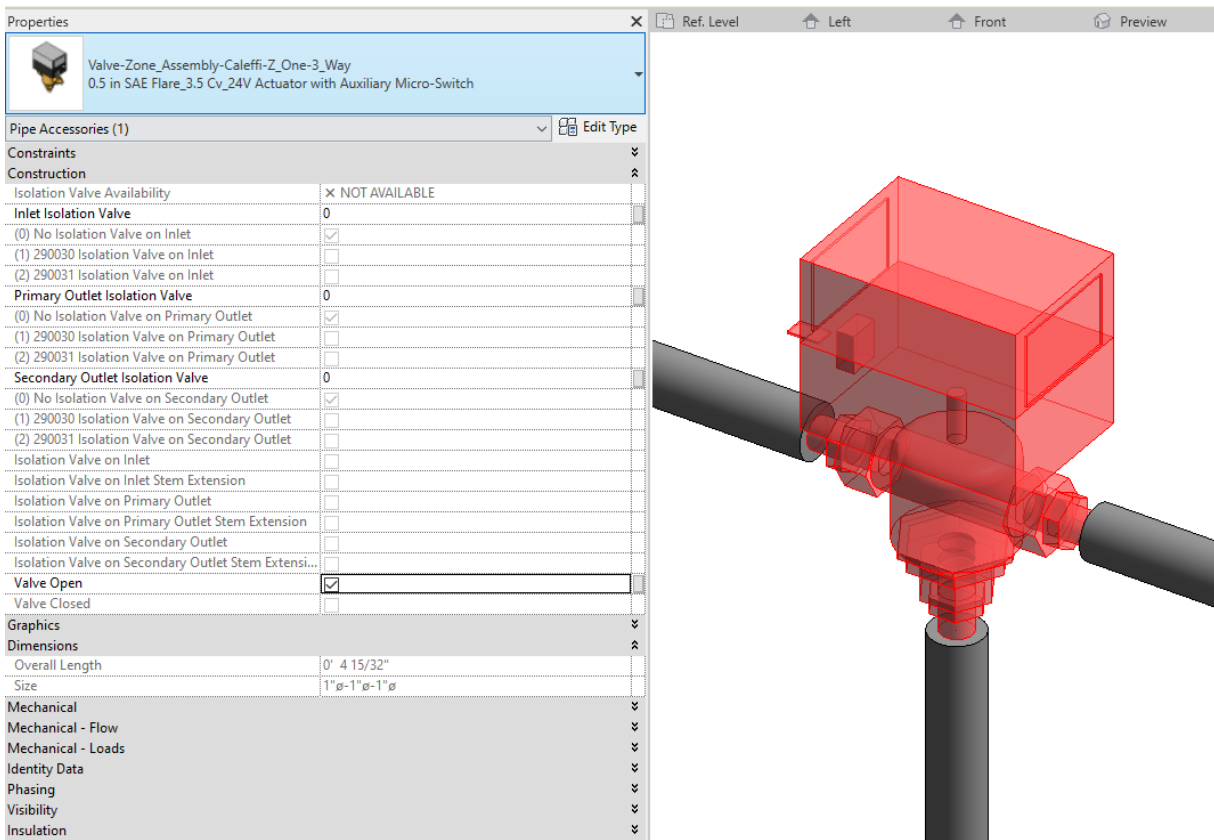
Figure 5 – The OBCaleffi Z-One Zone Valves families can be found under pipe accessories in the project browser and placed directly onto pipe of the same size. It will then read flows and consider pressure drop in the system.
